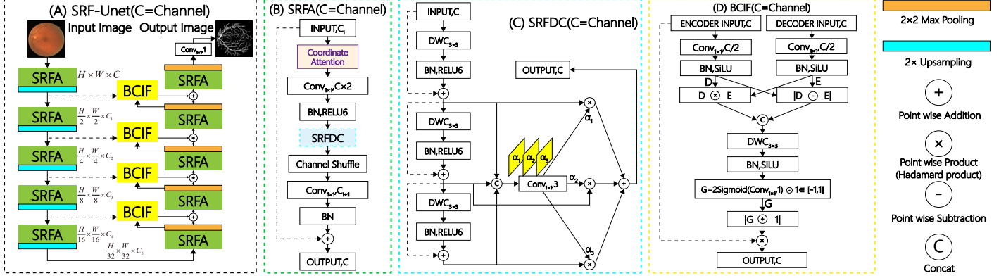
Figure 1. The proposed SRF-UNet architecture. (a) Five-stage SRF-UNet encoder-decoder, (b) serial residual fusion attention (SRFA), (c) serial residual fusion depthwise convolution (SRFDC), and (d) bipolar cross-interaction fusion (BCIF). C1–C5 denote the channel widths of the five encoder stages; [C1,C2,C3,C4,C5] is set to [8,16,32,48,80], [16,32,64,96,160], and [32,64,128,192,320] for SRF-UNet-S, SRF-UNet, and SRF-UNet-L, respectively. CA denotes Coordinate Attention[10]; DWC denotes depthwise convolution; BN denotes batch normalization.
